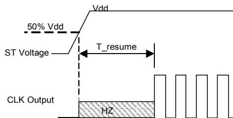
Figure 5. Standby Resume Timing (ST Mode Only)
